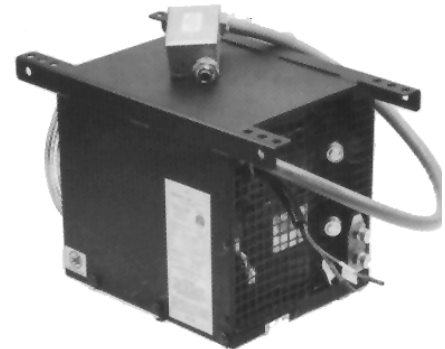
CONDENSING UNIT CN-8000
